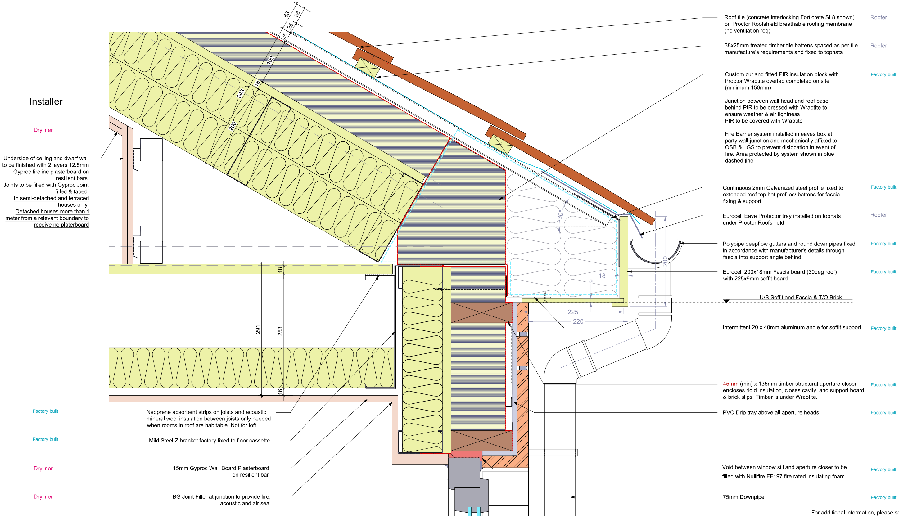
Roof Eaves Detail
