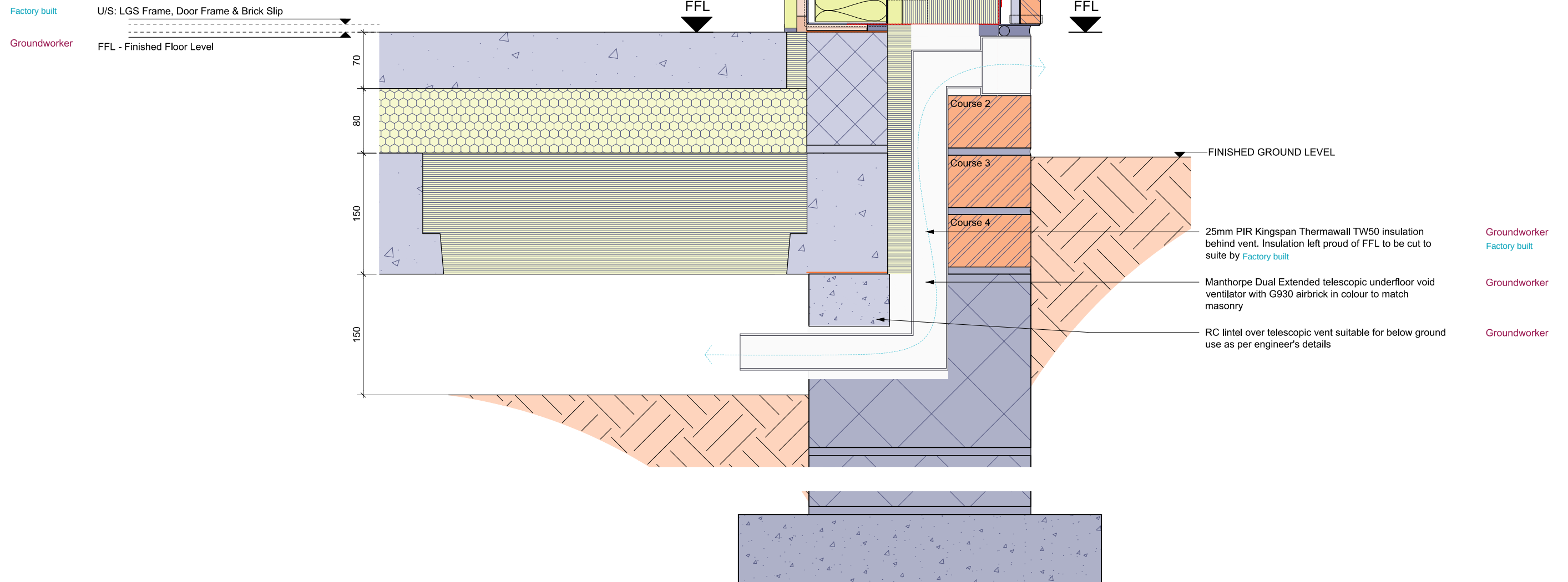
External Wall DPC Detail with Underfloor Vent (See DE001 for further information)
